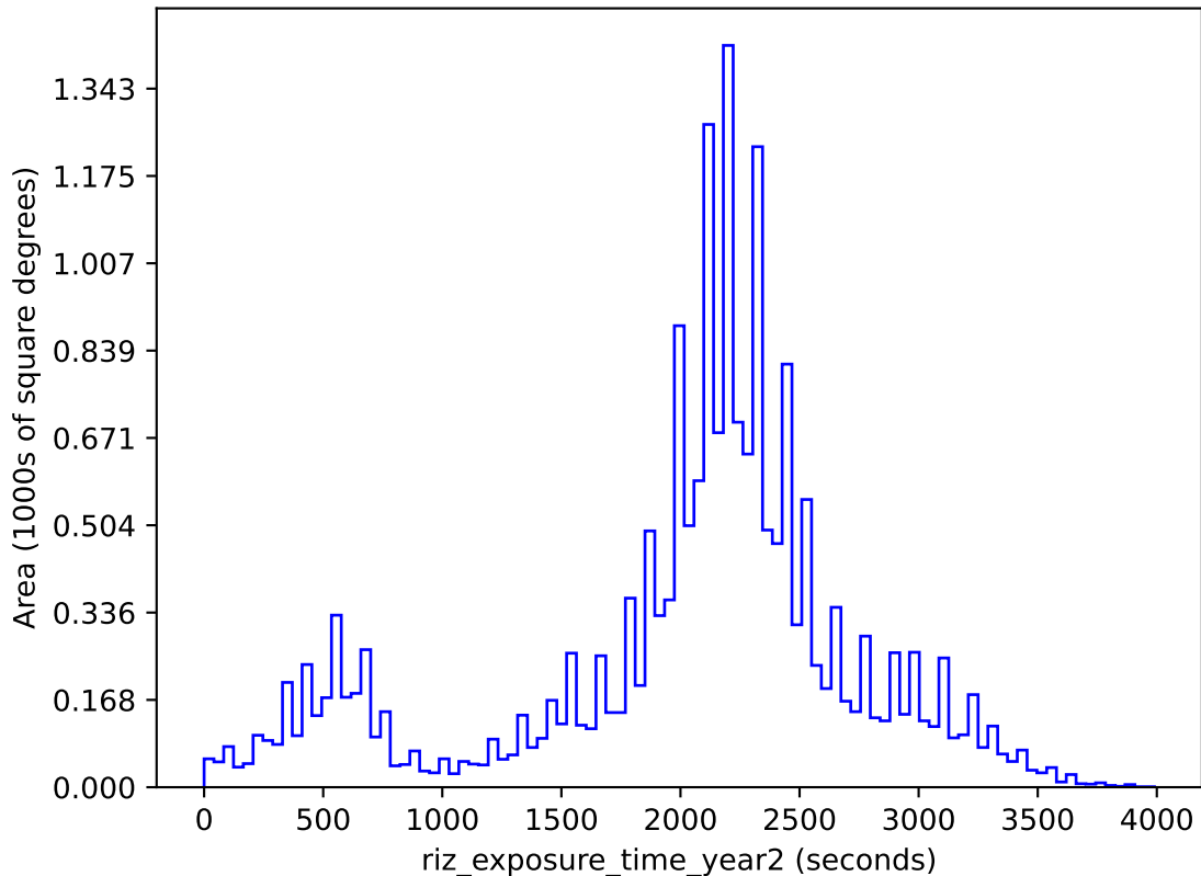
too_100_4v3.4_10yrs gri band non-DD: riz_exposure_time_year2
