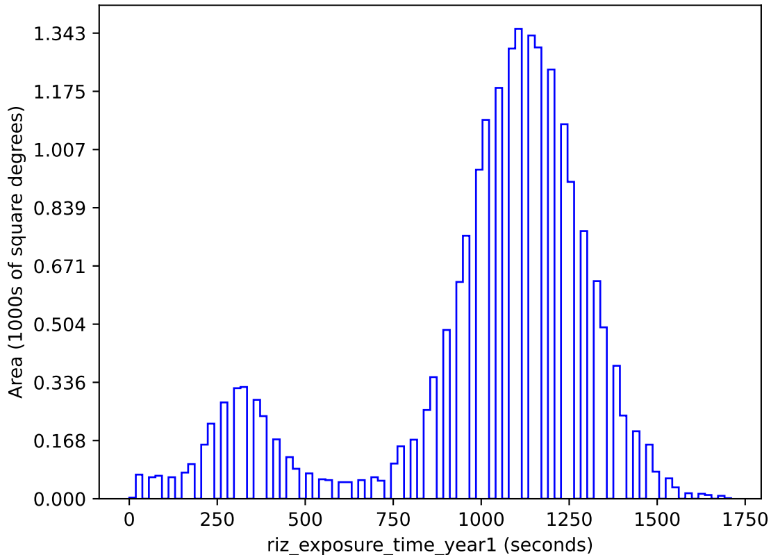
too_100_4v3.4_10yrs gri band non-DD: riz_exposure_time_year1
