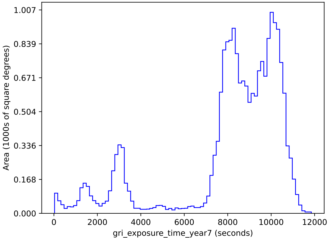
too_100_4v3.4_10yrs gri band non-DD: gri_exposure_time_year7
