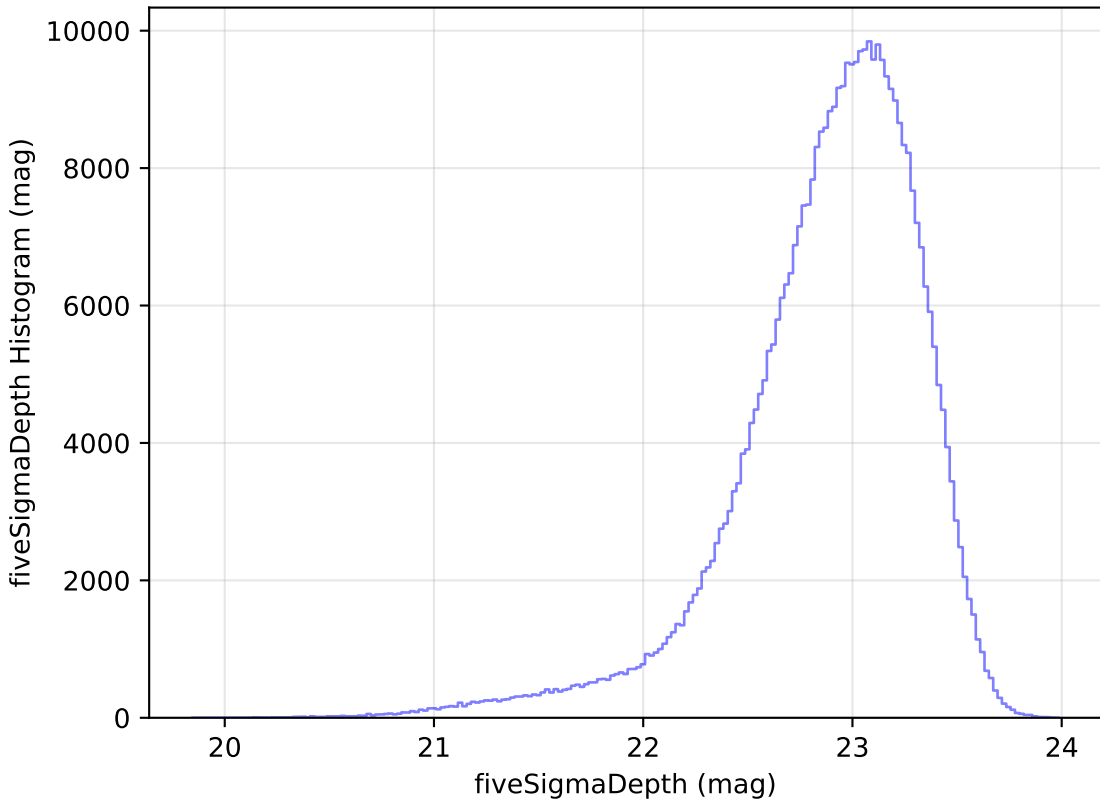
too_100_4v3.4_10yrs z: fiveSigmaDepth Histogram
