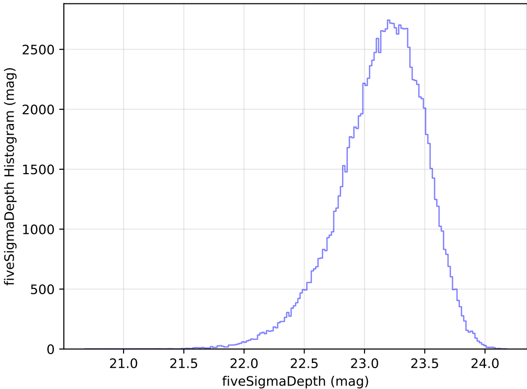
too_100_4v3.4_10yrs u: fiveSigmaDepth Histogram
