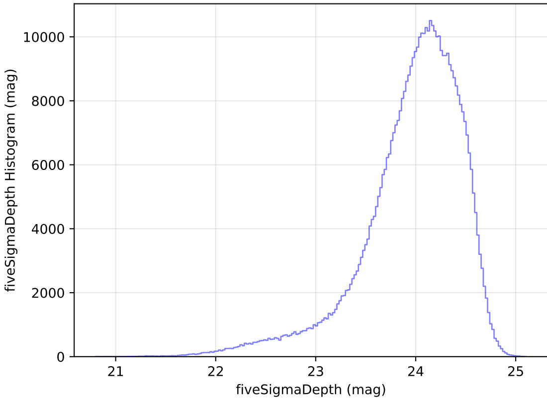
too_100_4v3.4_10yrs r: fiveSigmaDepth Histogram
