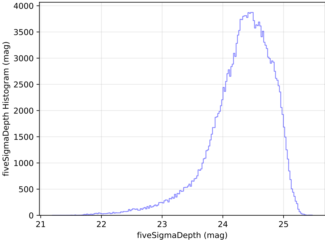
too_100_4v3.4_10yrs g: fiveSigmaDepth Histogram
