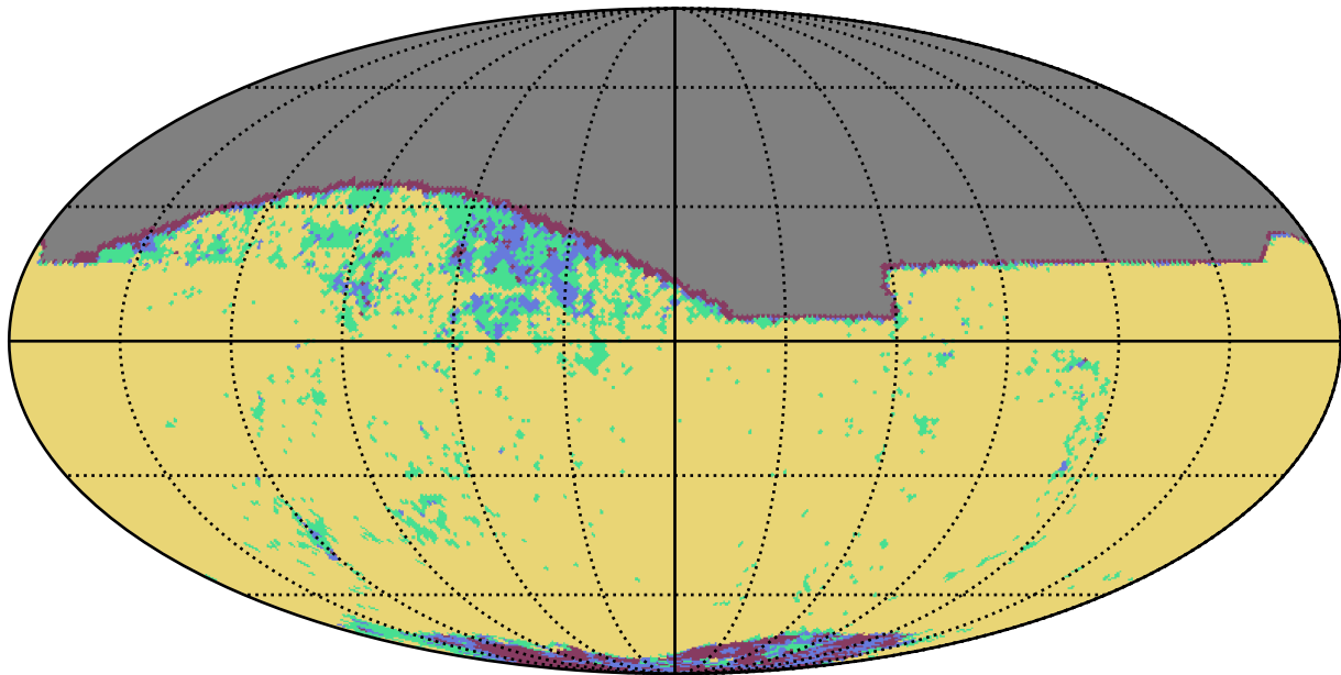
too_100_4v3.4_10yrs z band: YearCoverage night
