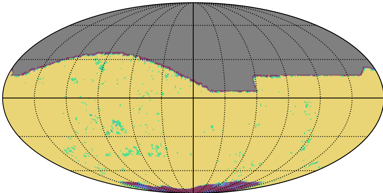
too_100_4v3.4_10yrs r band: YearCoverage night
