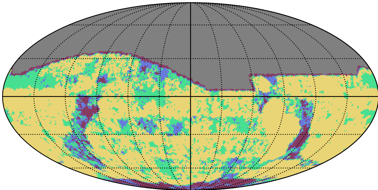
too_100_4v3.4_10yrs g band: YearCoverage night
