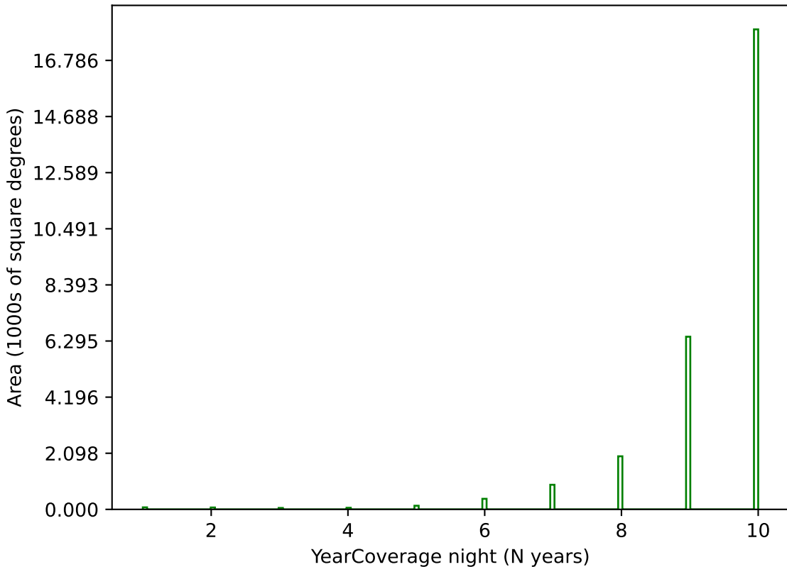
too_100_4v3.4_10yrs g band: YearCoverage night
