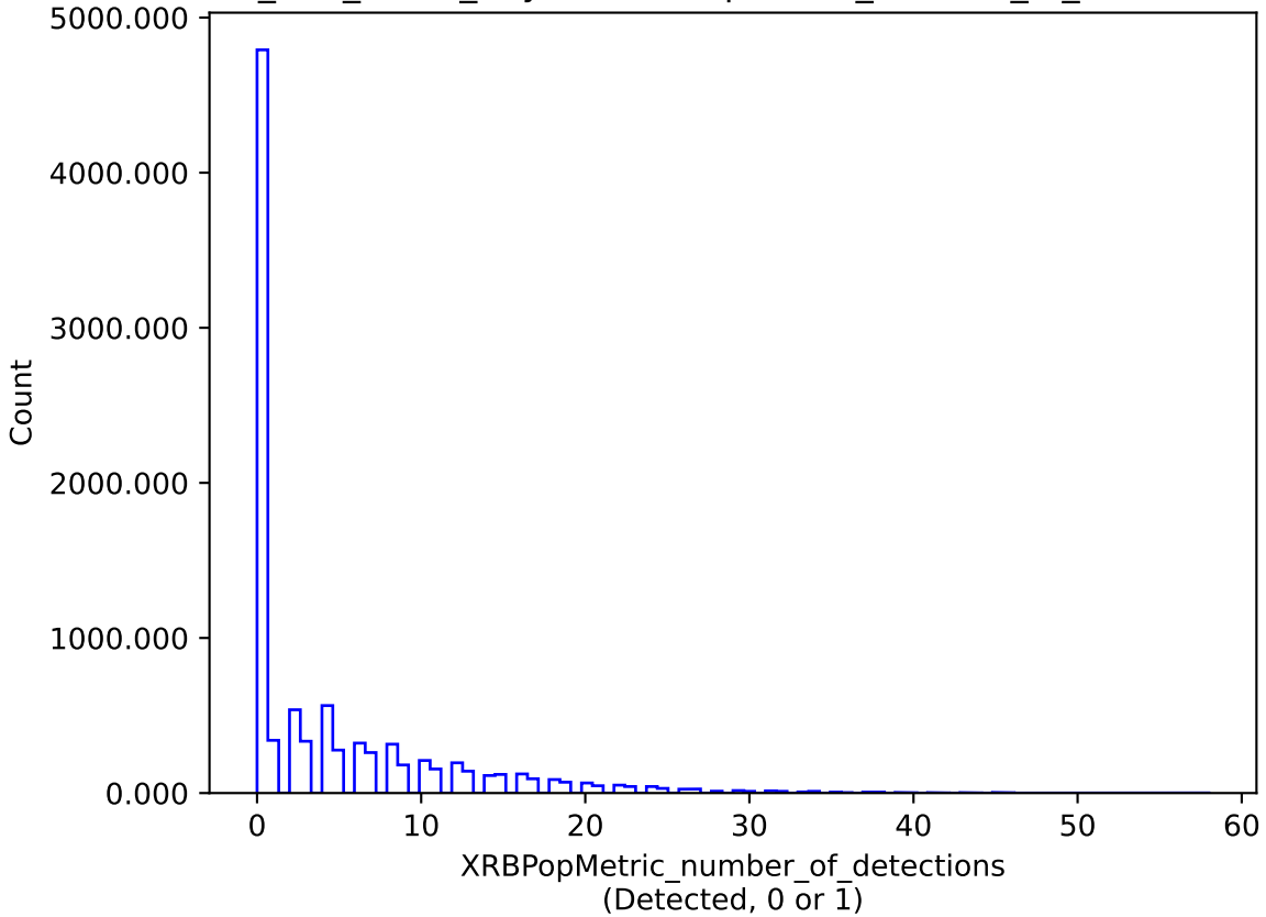
too_100_4v3.4_10yrs : XRBPoMetric_number_of_detections
