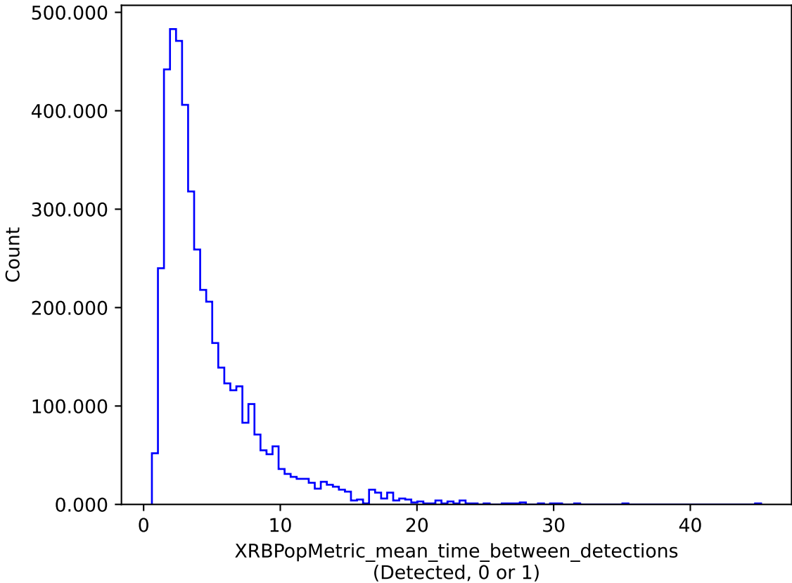
too_100_4v3.4_10yrs : XRBPopMetric_mean_time_between_detections
