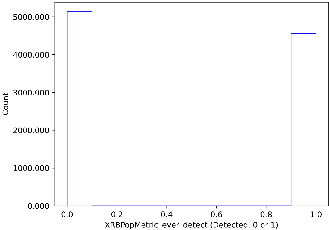
too_100_4v3.4_10yrs : XRBPoMetric_ever_detect
