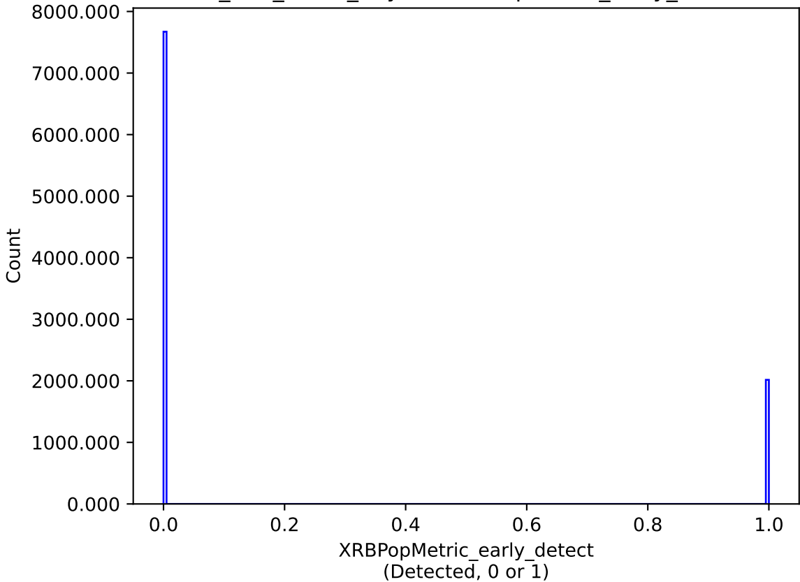
too_100_4v3.4_10yrs : XRBPoMetric_early_detect
