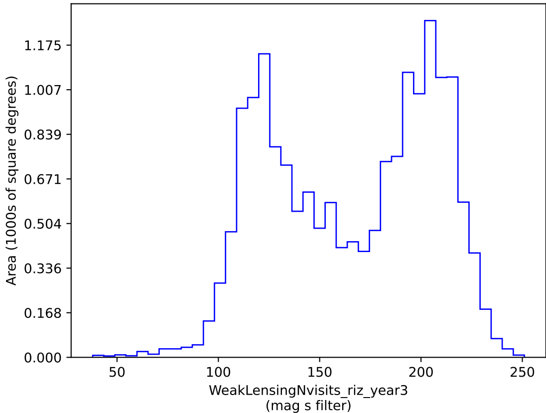
too_100_4v3.4_10yrs gri band non-DD: WeakLensingNvisits_riz_year3
