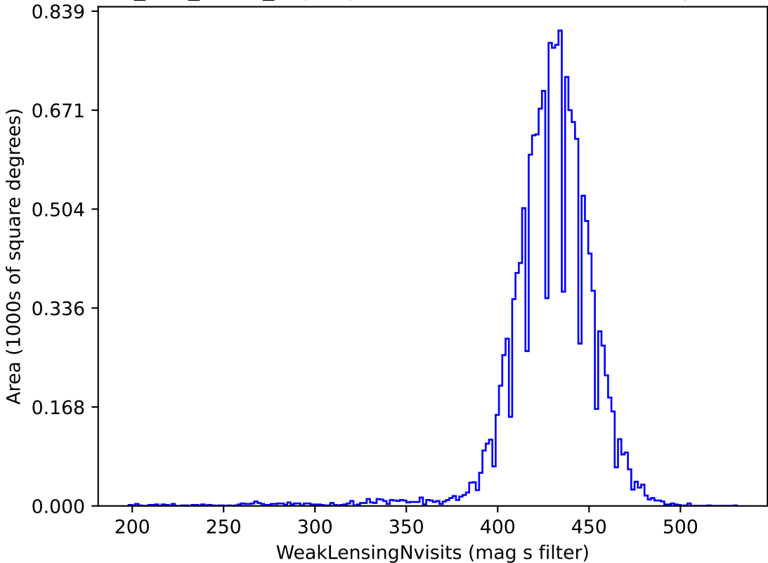
too_100_4v3.4_10yrs gri band non-DD: WeakLensingNvisits
