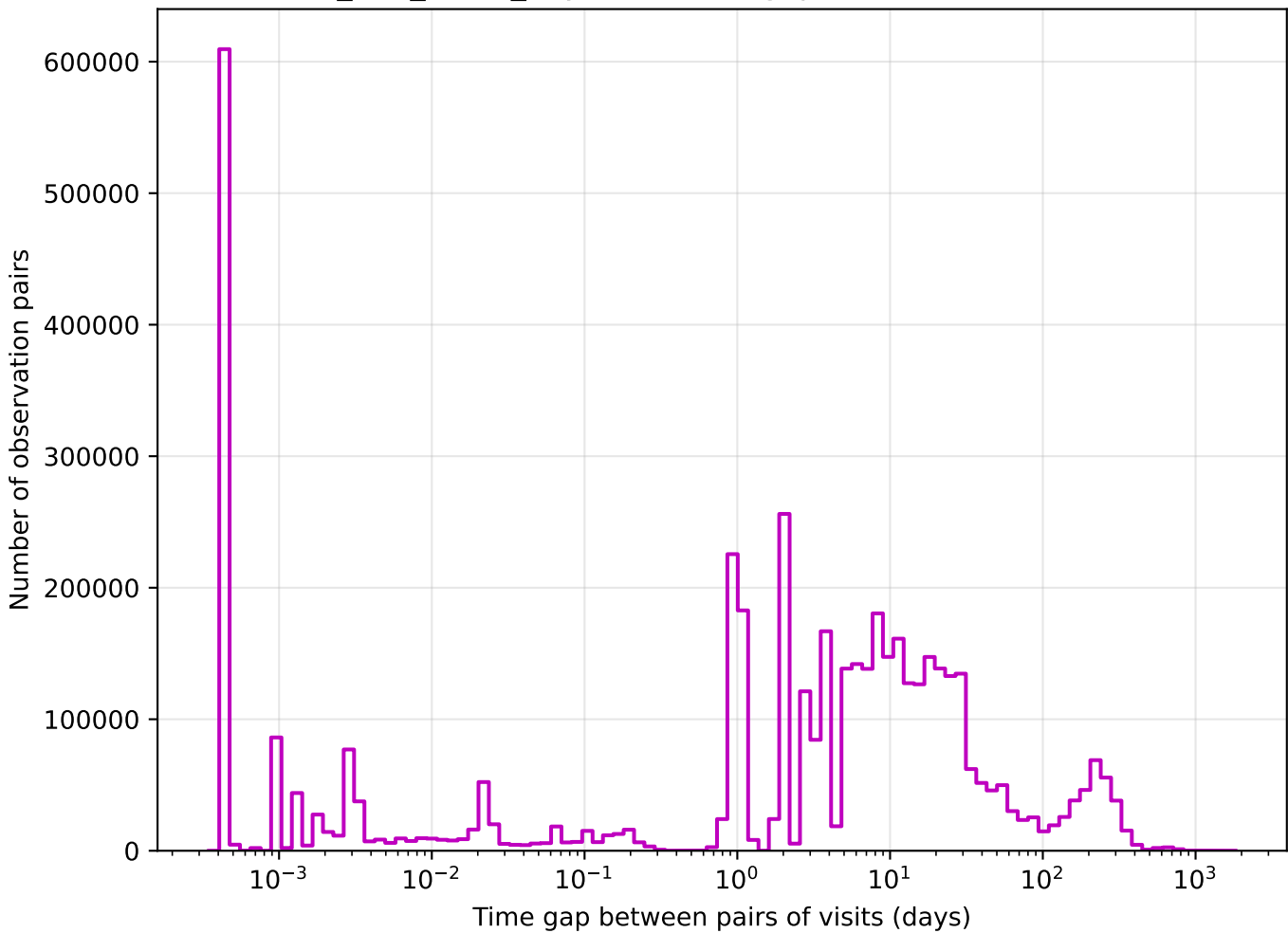
too_100_4v3.4_10yrs z band: Tgaps observationStartMJD
