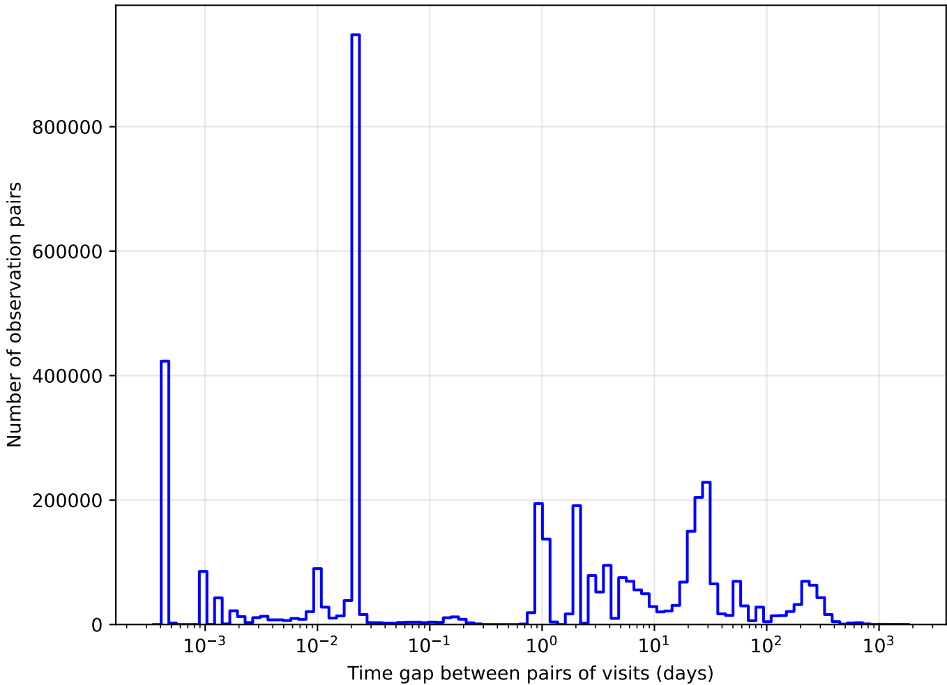
too_100_4v3.4_10yrs y band: Tgaps observationStartMJD
