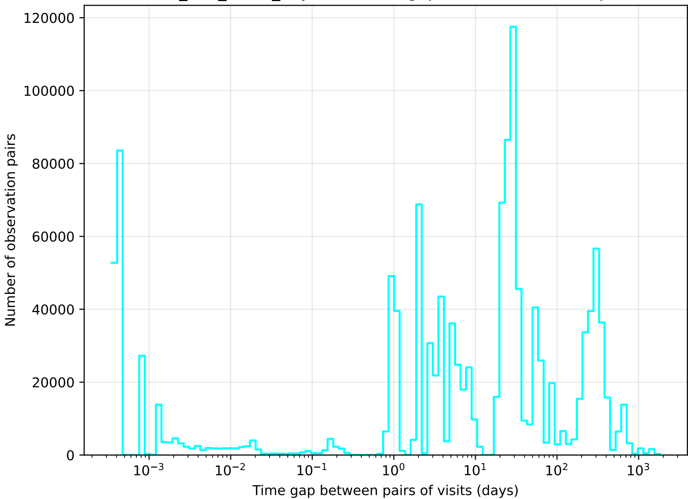
too_100_4v3.4_10yrs u band: Tgaps observationStartMJD
