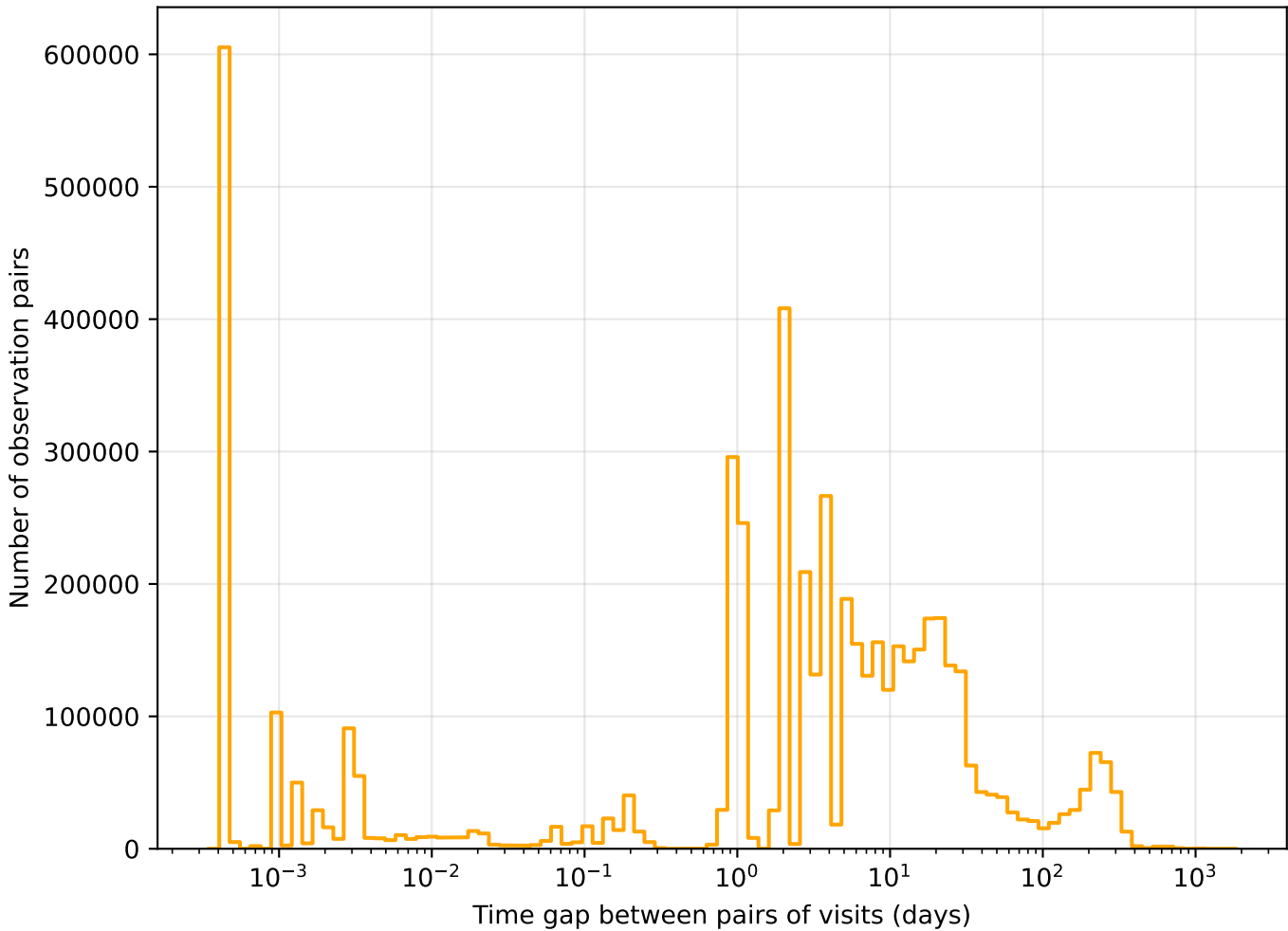
too_100_4v3.4_10yrs r band: Tgaps observationStartMJD
