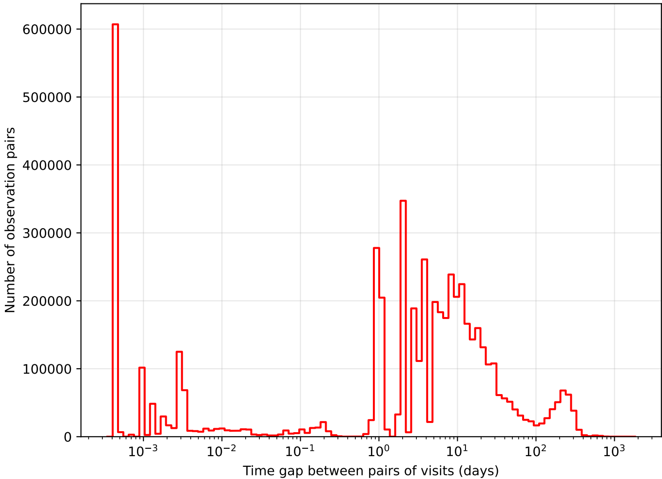
too_100_4v3.4_10yrs i band: Tgaps observationStartMJD
