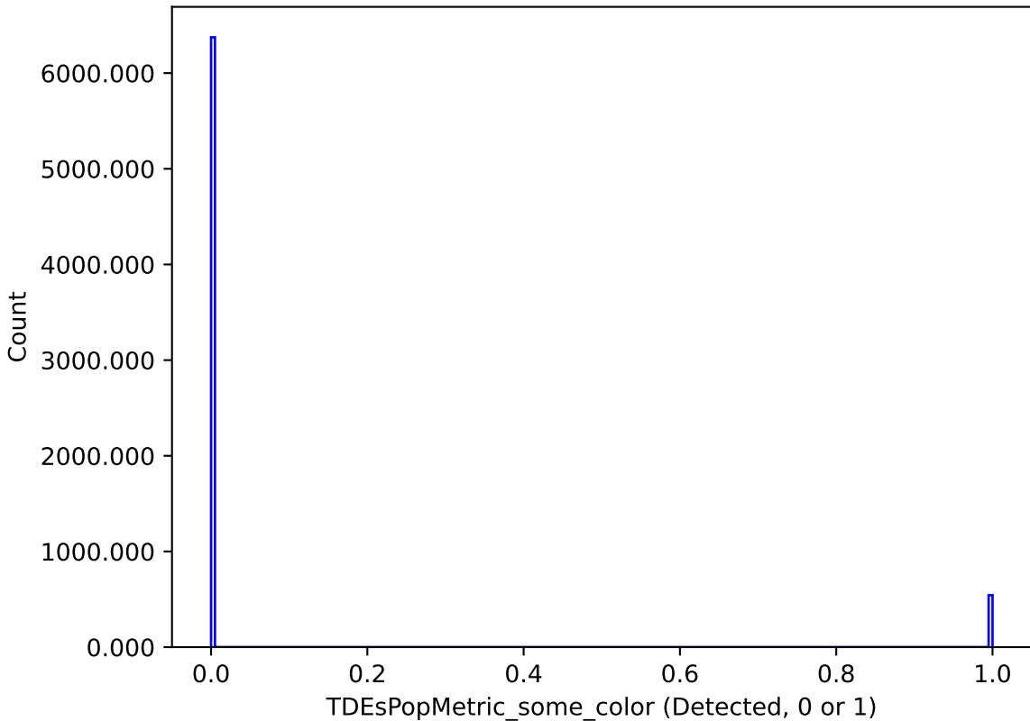
too_100_4v3.4_10yrs : TDEsPopMetric_some_color
