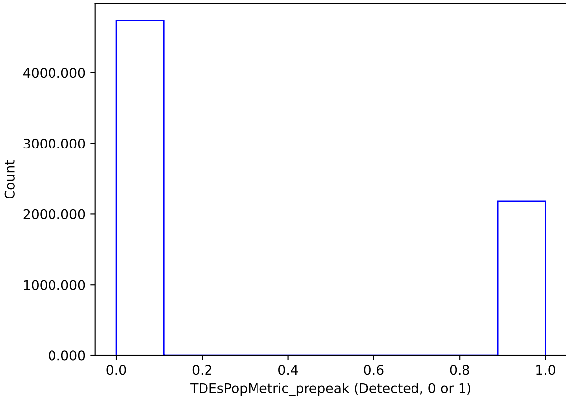
too_100_4v3.4_10yrs : TDEsPopMetric_prepeak
