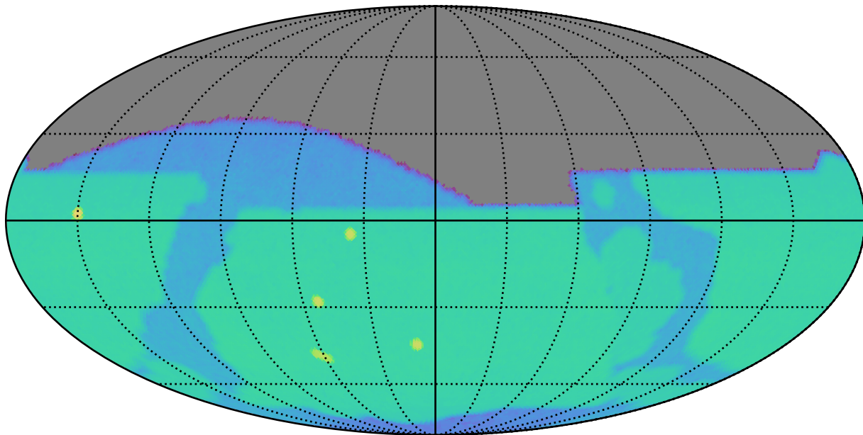
too_100_4v3.4_10yrs z: SurfaceBrightLimit
