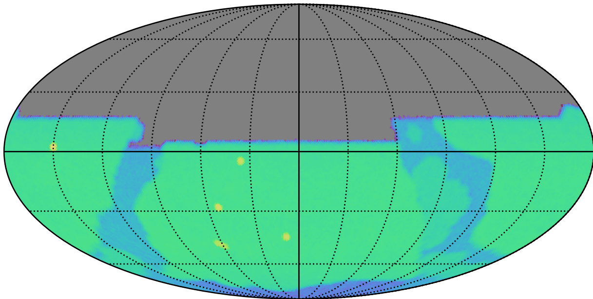
too_100_4v3.4_10yrs y: SurfaceBrightLimit
