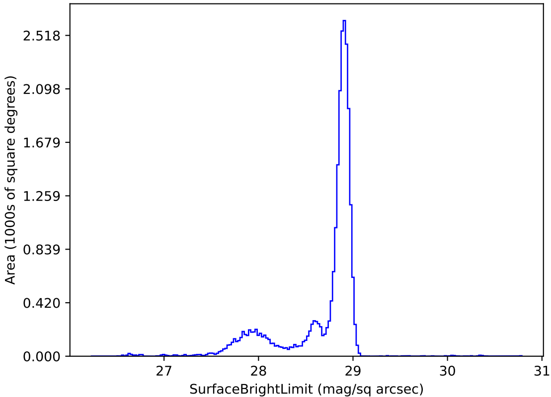
too_100_4v3.4_10yrs u: SurfaceBrightLimit
