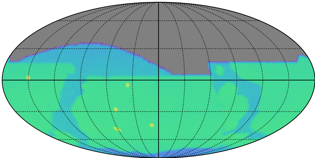
too_100_4v3.4_10yrs r: SurfaceBrightLimit
