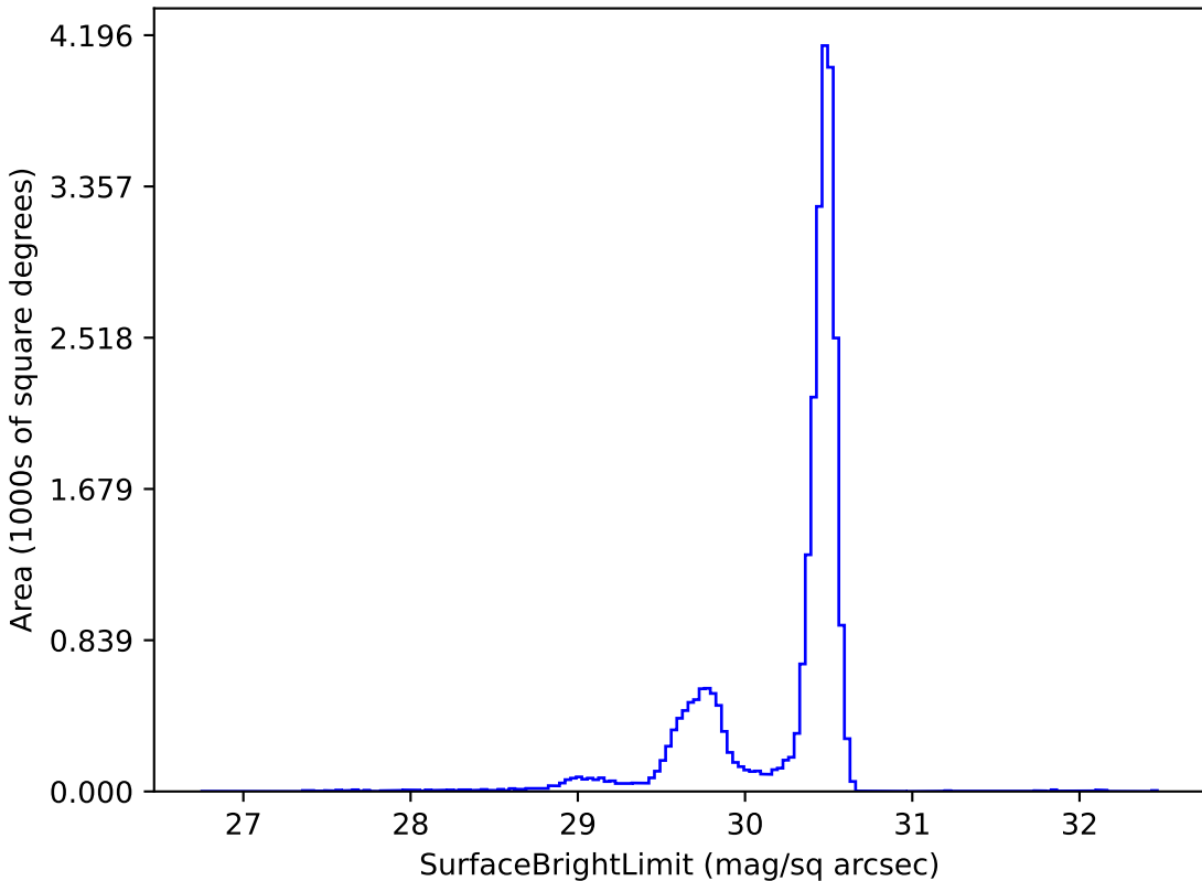
too_100_4v3.4_10yrs r: SurfaceBrightLimit
