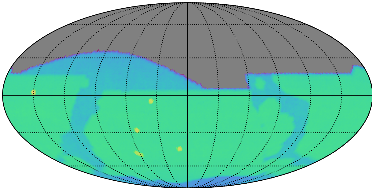
too_100_4v3.4_10yrs i: SurfaceBrightLimit
