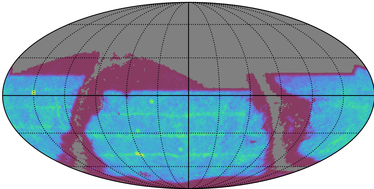
too_100_4v3.4_10yrs : SNSLMetric
