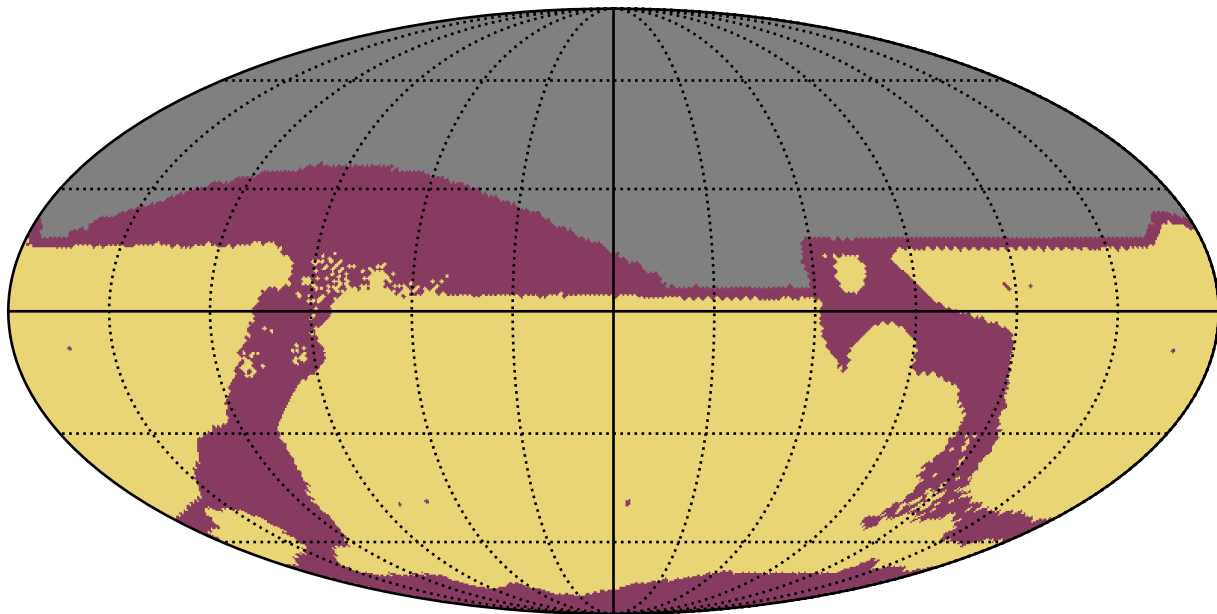
too_100_4v3.4_10yrs : RapidRevisits
