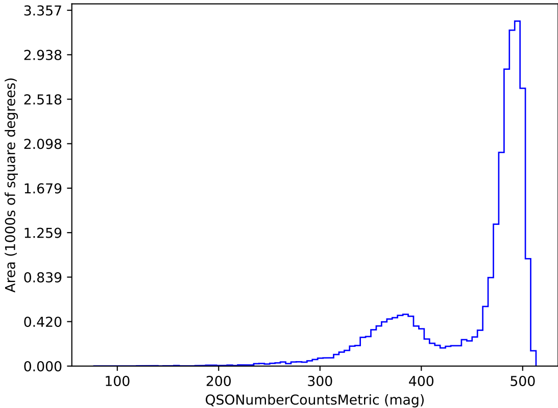
too_100_4v3.4_10yrs z band and non-DD: QSONumberCountsMetric
