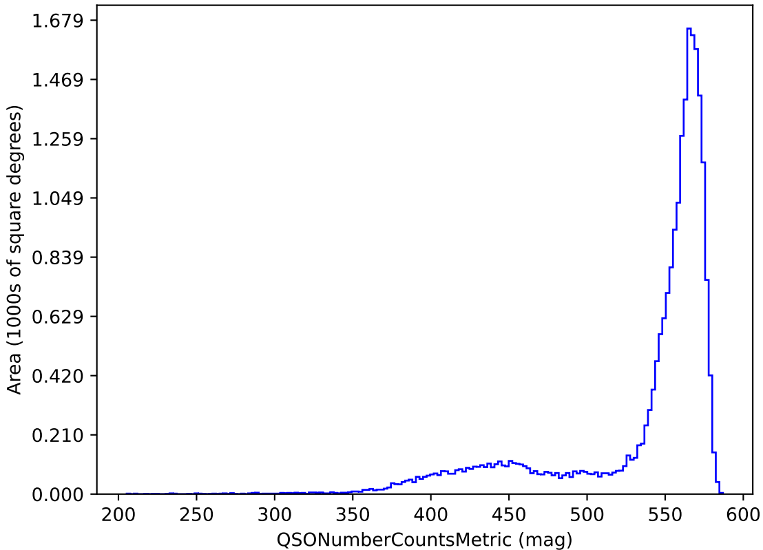
too_100_4v3.4_10yrs y band and non-DD: QSONumberCountsMetric
