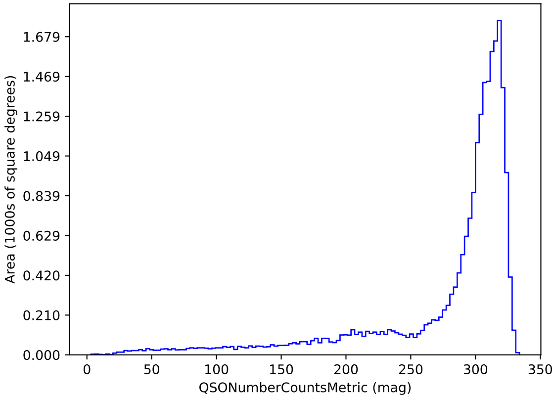
too_100_4v3.4_10yrs u band and non-DD: QSONumberCountsMetric
