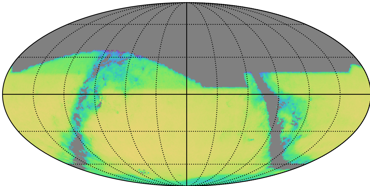
too_100_4v3.4_10yrs r band and non-DD: QSONumberCountsMetric
