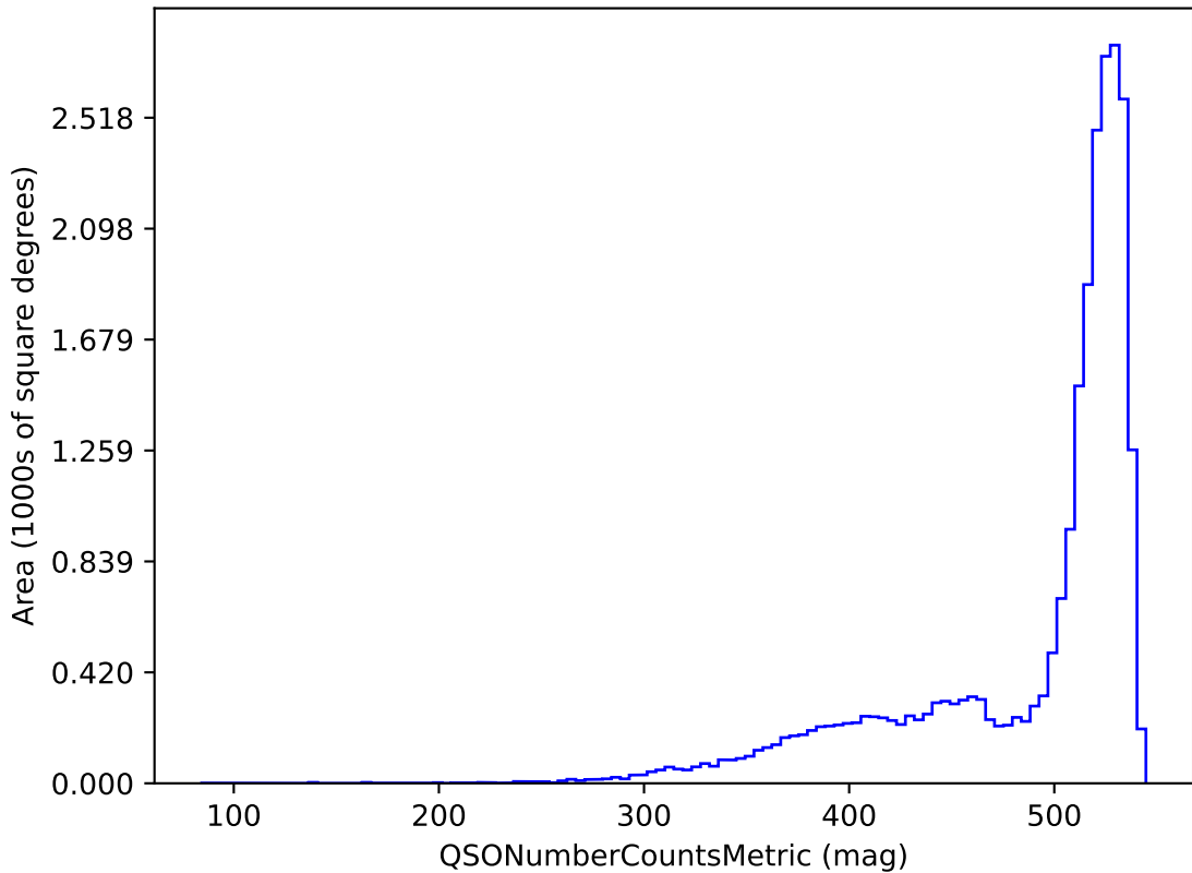
too_100_4v3.4_10yrs r band and non-DD: QSONumberCountsMetric
