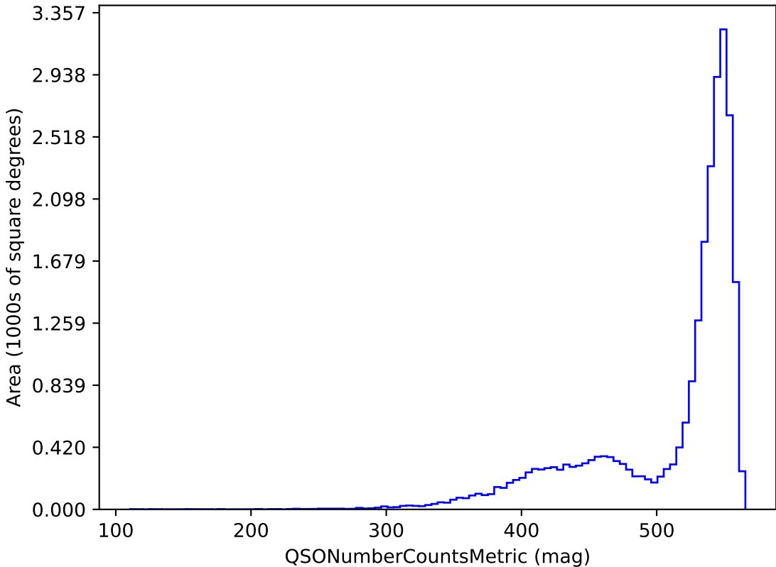
too_100_4v3.4_10yrs i band and non-DD: QSONumberCountsMetric
