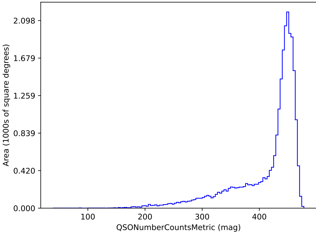
too_100_4v3.4_10yrs g band and non-DD: QSONumberCountsMetric
