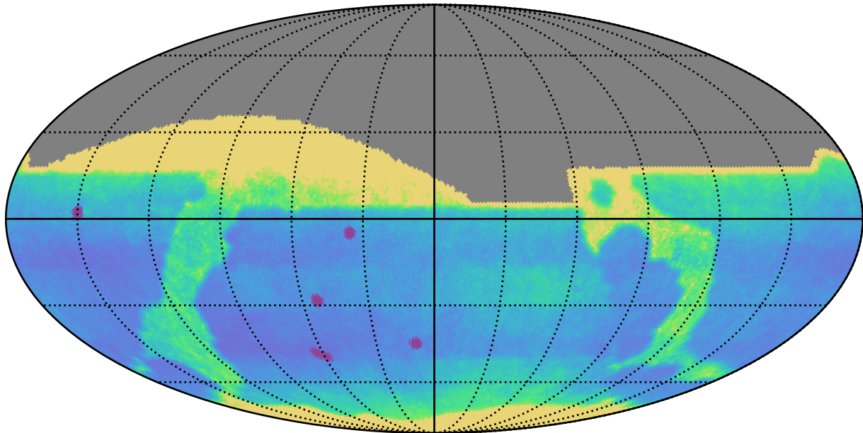
too_100_4v3.4_10yrs : Proper Motion Uncert @ 24.0
