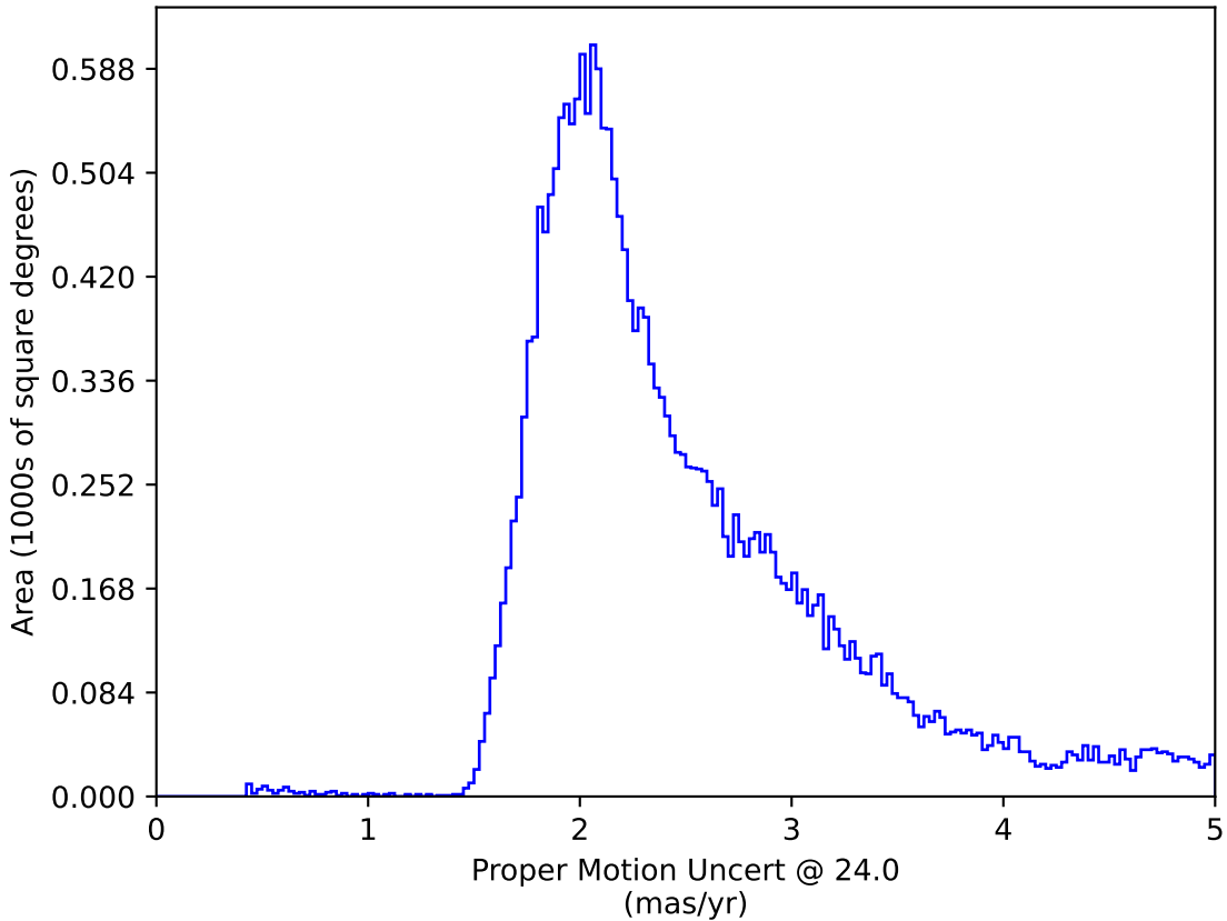
too_100_4v3.4_10yrs : Proper Motion Uncert @ 24.0
