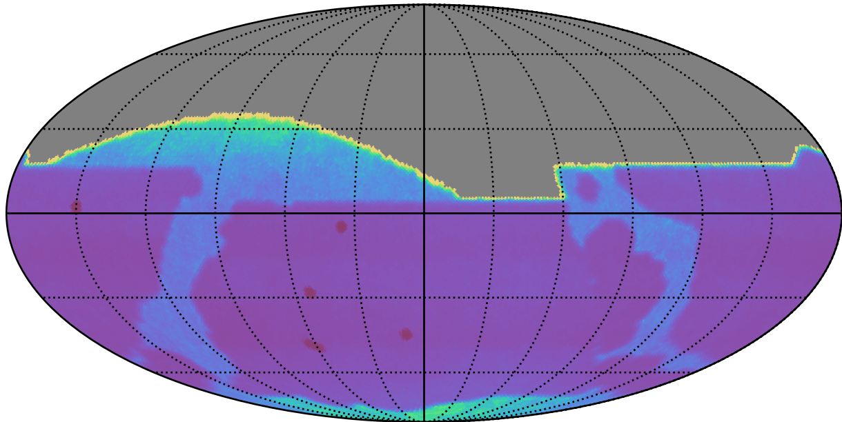
too_100_4v3.4_10yrs : Proper Motion Uncert @ 20.5
