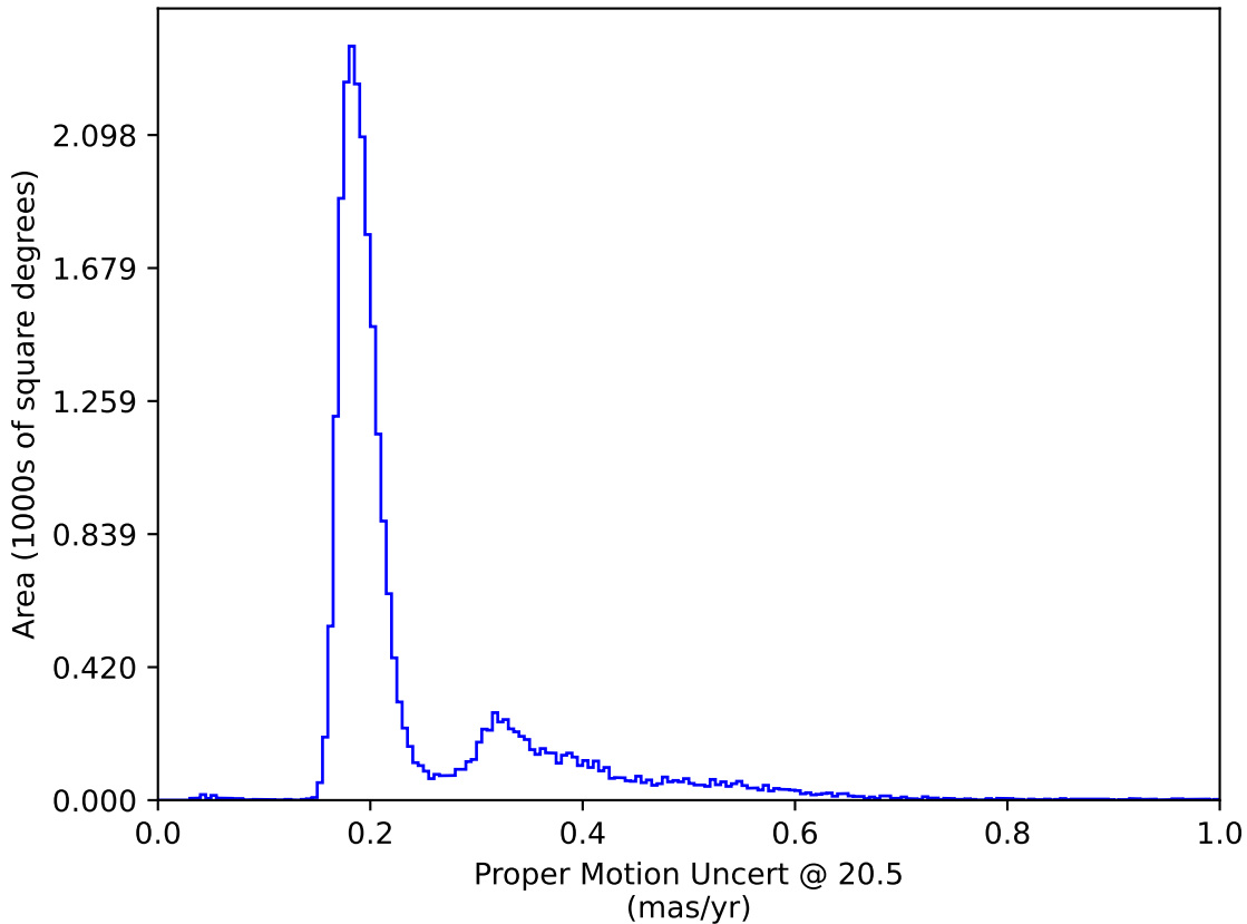
too_100_4v3.4_10yrs : Proper Motion Uncert @ 20.5
