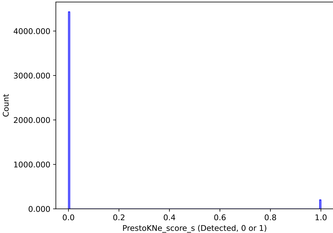
too_100_4v3.4_10yrs : PrestoKNe_score_s
