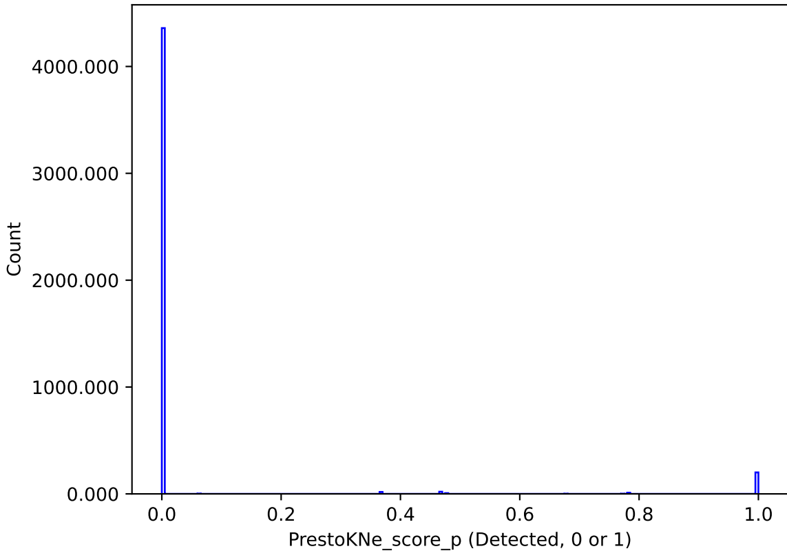
too_100_4v3.4_10yrs : PrestoKNe_score_p
