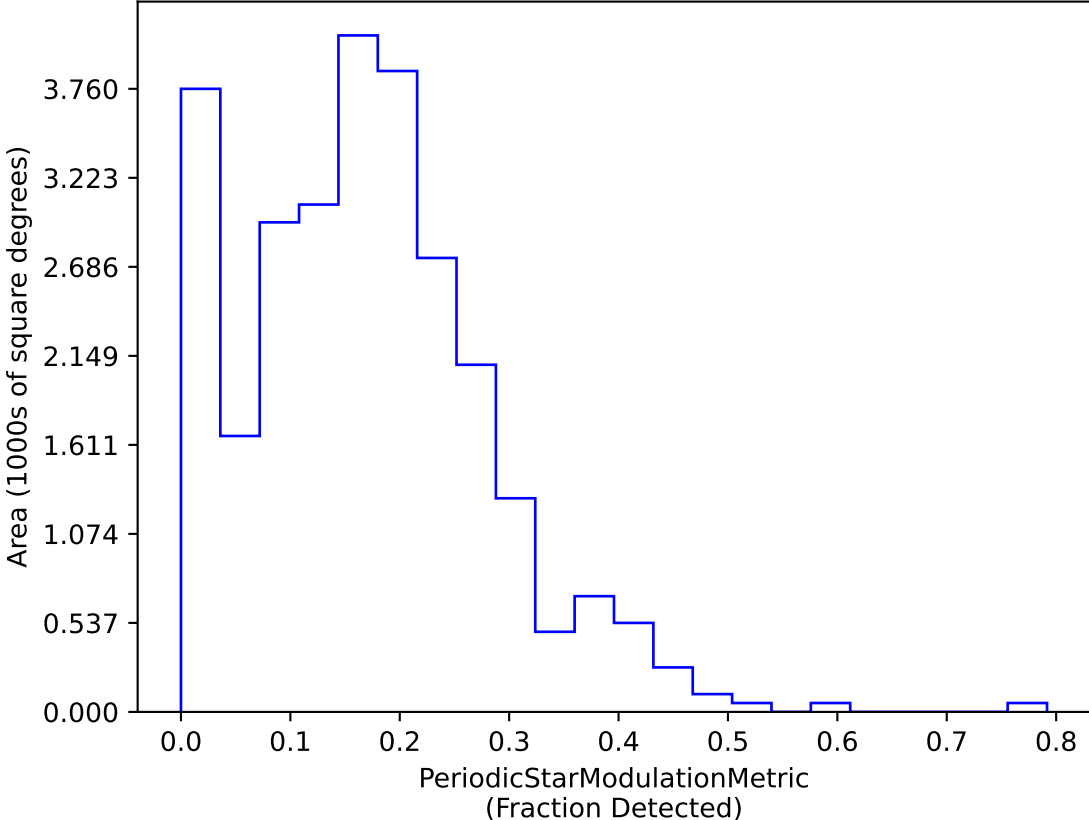
too_100_4v3.4_10yrs dm 18 interval 15 RRC Year 1-2: PeriodicStarModulationMetric
