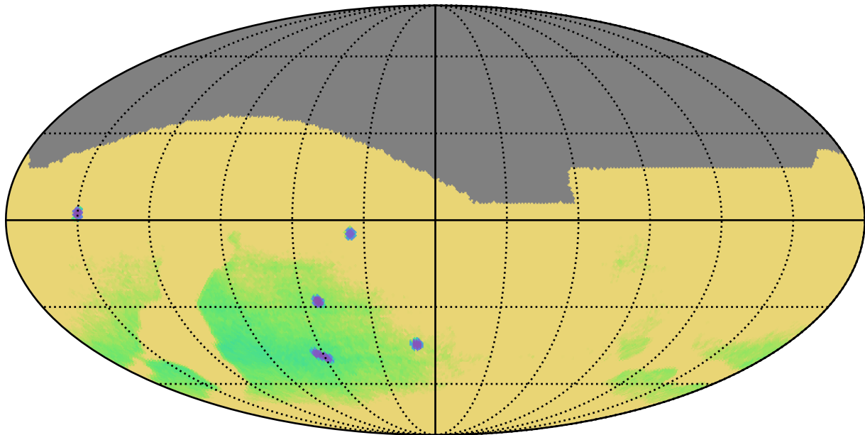
too_100_4v3.4_10yrs : Parallax Uncert @ 22.4
