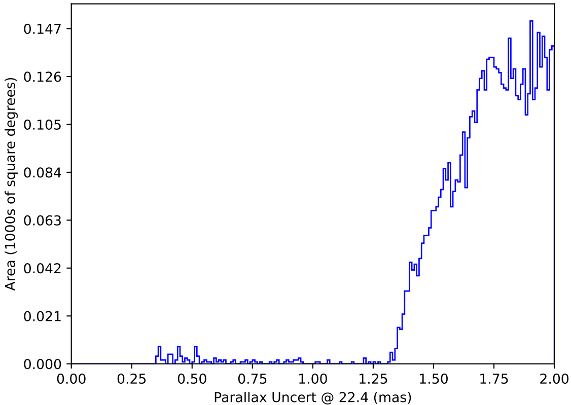
too_100_4v3.4_10yrs : Parallax Uncert @ 22.4
