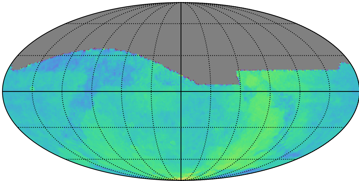
too_100_4v3.4_10yrs : Parallax Coverage @ 22.4
