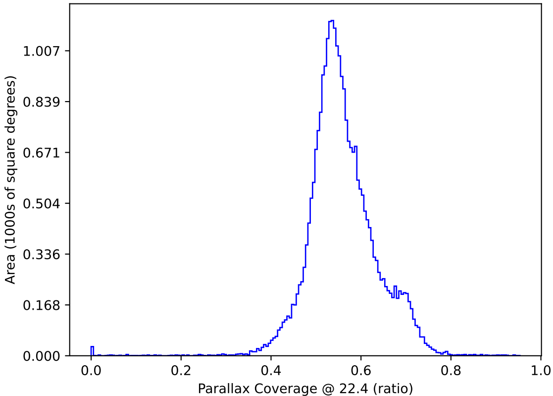
too_100_4v3.4_10yrs : Parallax Coverage @ 22.4
